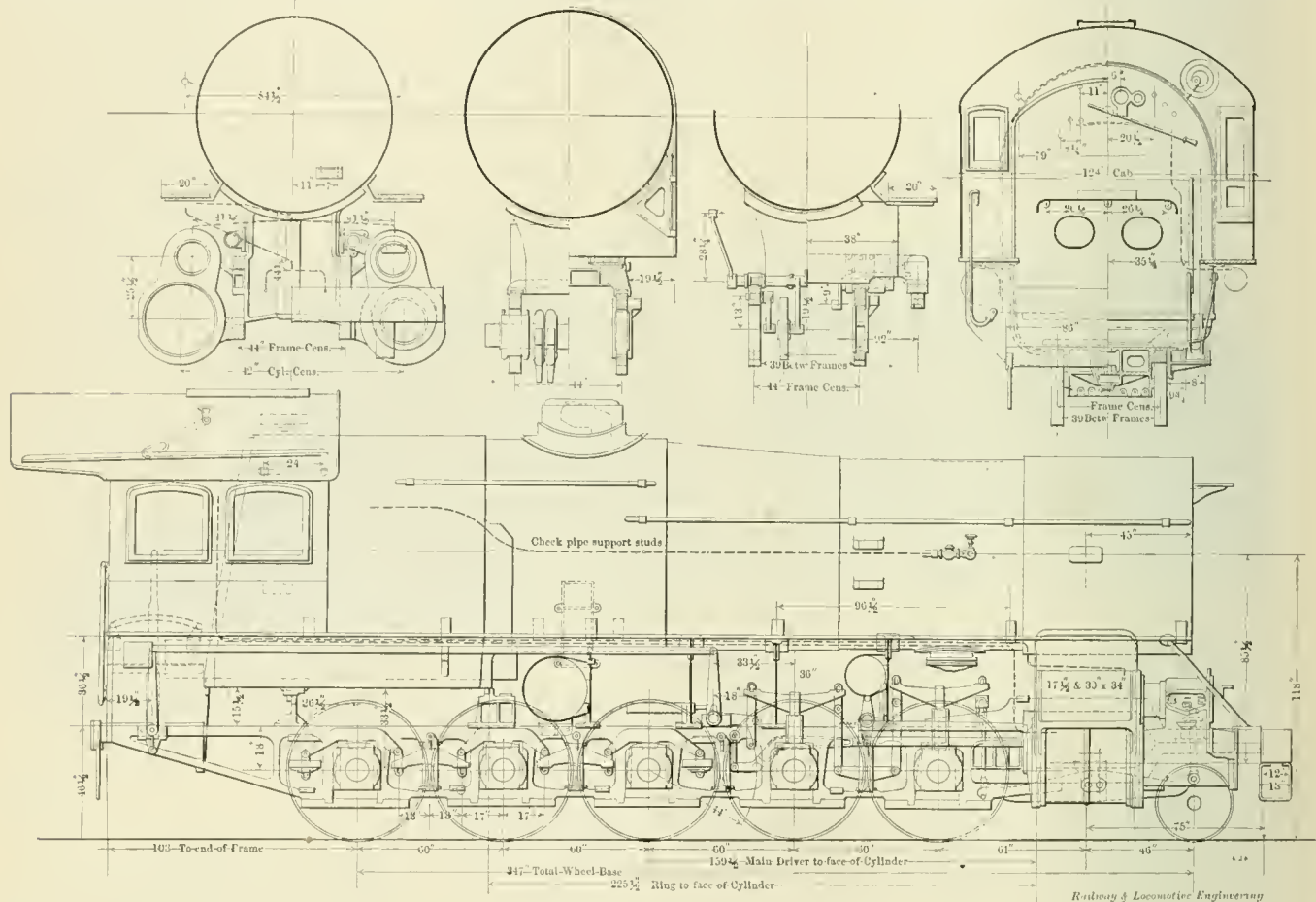
THE LARGEST ENGINE YET BUILT.
